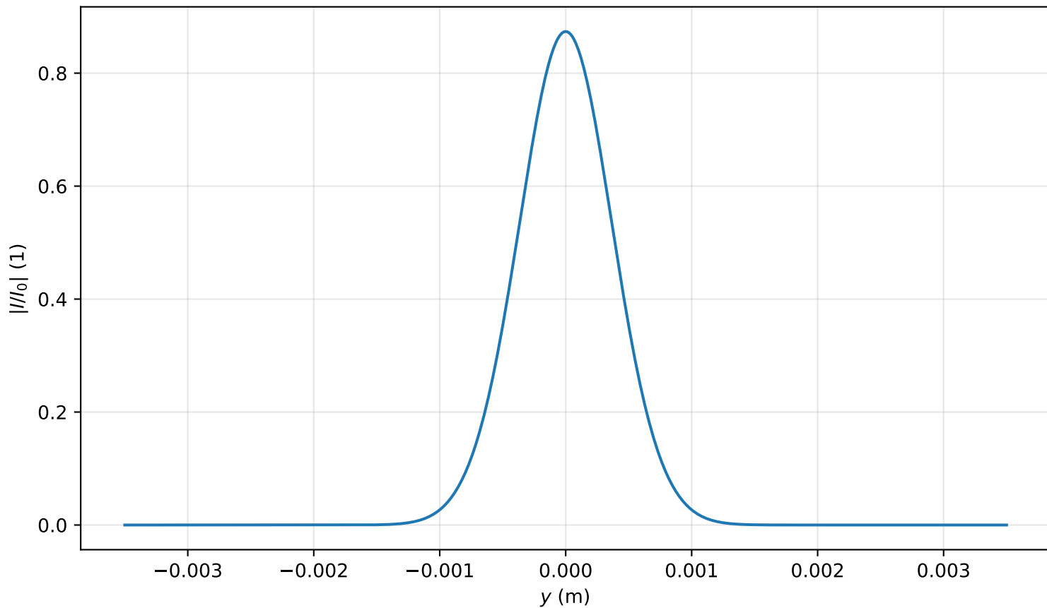
Intensity profile I(x=0, y, z=0.876)/I_0 , P_{in}=0.1P_{cr} , artificial time
